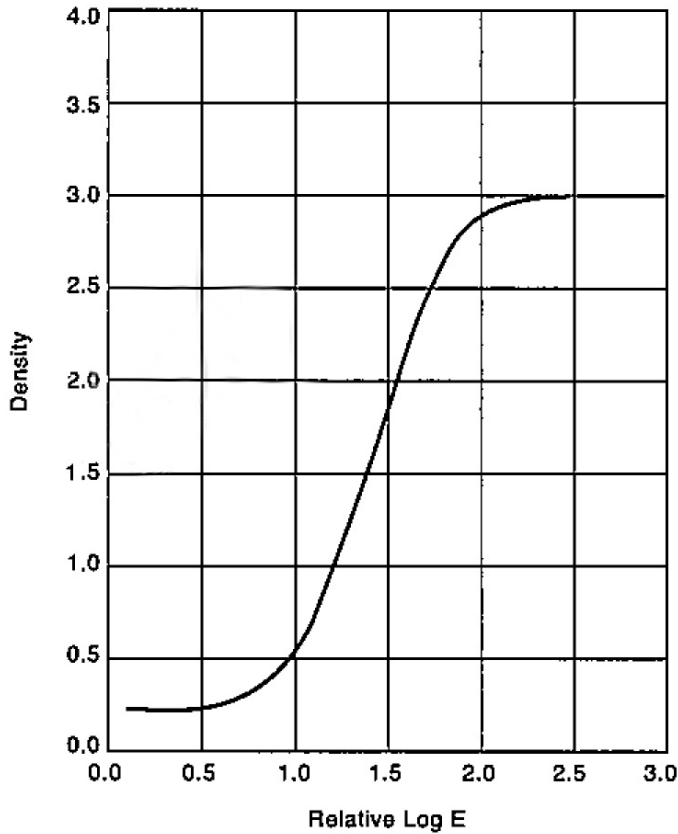
Fig. 3 Characteristic Curve
